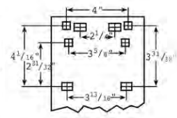
Rear Mount
