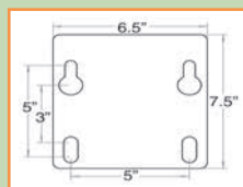
GBA-180 Mounting Plate
