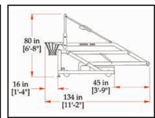
PBEL66 folded dimensions
