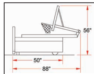
PBB-200 folded dimensions
