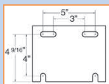
GBA-342A Mounting Plate GBA-600 Mounting Plate
