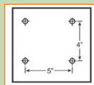
GBA-18042 Mounting Plate
