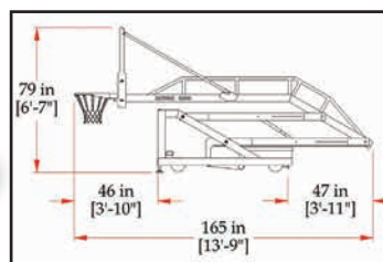
PBEL96 folded dimensions
