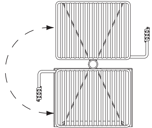
Grate rotates 180° out of the fire. The grate handle is never over the fire.
