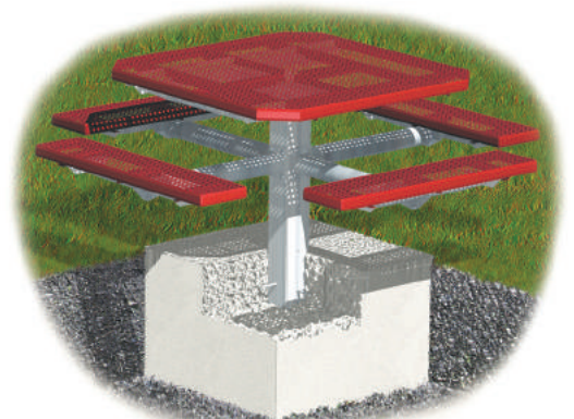
Model PQT/G-4HR showing standard embedded post installation, galvanized frames, 48" top, red thermo-plastic coated perforated steel.
