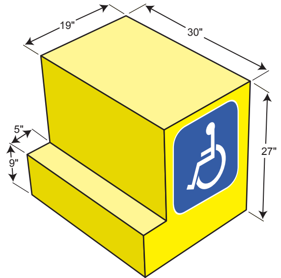
The ADA Clearance Box fits completely underneath the W Series table end. This Pilot Rock table provides all the required vertical and horizontal knee and toe clearances. (Note: this unique table design is covered under 6 patents.)
