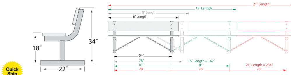
Aluminum Curved Back Bench
