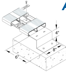
Model #1119Z-S Stadium Bench "Z" Bracket without Back
