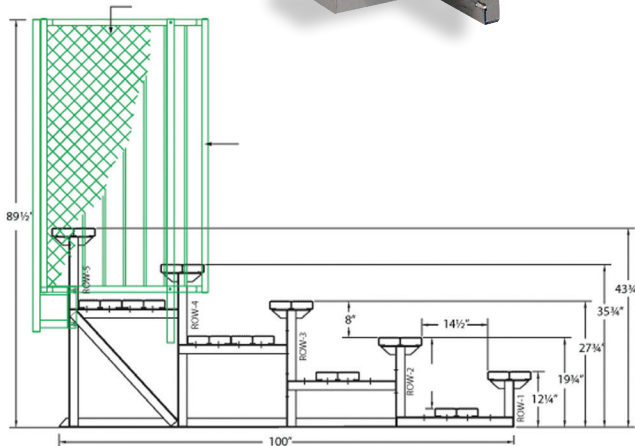
STANDARD 5-ROW BLEACHER DIMENSIONS
